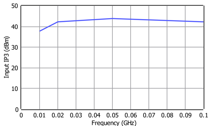
Input IP3 at Low Frequencies
