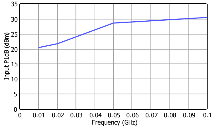
Input P1dB at Low Frequencies
